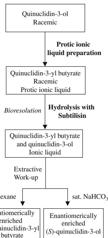
Figure 4. Facile processing for the bioresolution of racemic quinuclidin-3-ol.
